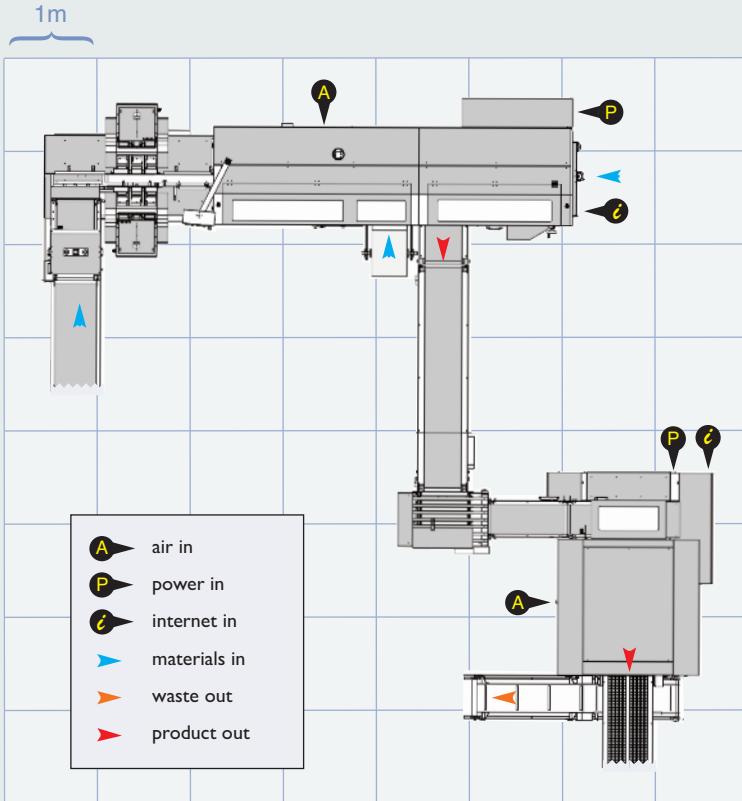
This sample floorplan shows the BRM-G single-clamp binder in-line with the TR30S 3-knife trimmer. The footprint alters according to the equipment specified. Conveyors can be supplied to create the optimum configuration for the specific production environment.
